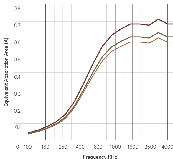
Absorption Coefficient according to ISO 354
